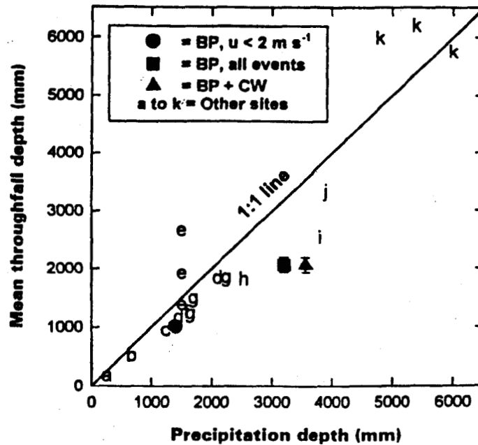
Figure 1. Annual precipitation depth (mm) versus mean throughfall depth (mm) at selected premontane and TMF sites. Symbols represent TF depth (mean mm \pm SE) at Monteverde, letters are other sites; a = Juvic & Nullet (1995), b = Cavalier & Goldstein (1989), c = Lundgren & Lundgren (1979), d = Veneklaas & Van Ek (1990), e = Stadtmuller & Aguedelo (1990), f = Steinhardt (1979), g = Vis (1986), h = Clements & Colon (1975), i = Edwards (1982), j = Mamanteo & Veracion (1985), k = Weaver (1972).
