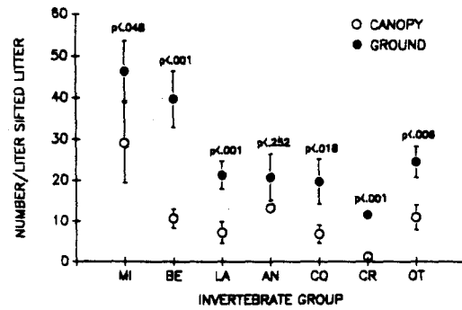
FIGURE 1. Invertebrate density (number of individuals/liter of sifted litter) by invertebrate group for ground and canopy samples. MI = mires, BE = adult beetles, LA = holometabolous insect larvae, AN = adult ants, CO = Collembola, CR = amphipods and isopods, OT = other (Hemiptera, Homoptera, Orthoptera, Dictyoptera, Dermaptera, adult Diptera, Thysanoptera, parasitic Hymenoptera, Apterygota, Symphyla, millipeds, centipeds, spiders, other Arachnida, Gastropoda, Annelida). Significance values above categories are results of paired-sample t -tests. Error bars represent two standard errors of the means.
